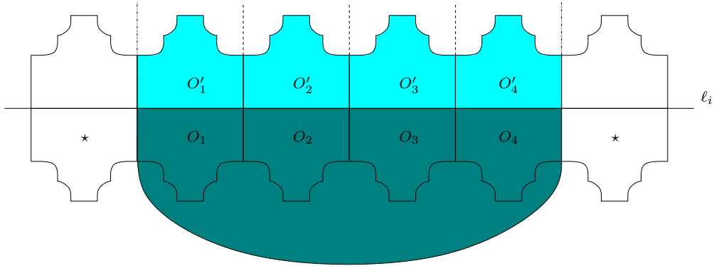
FIG. 4.1. From \widetilde{\mathcal{M}}_{i-1} (dark shaded) to \widetilde{\mathcal{M}}_i (all shaded).
