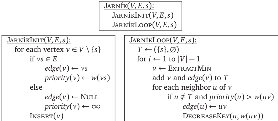
Figure 7.5. Jarník's minimum spanning tree algorithm, ready to be used with a Fibonacci heap
