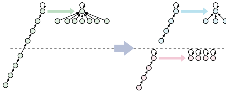
A COMPRESS operation in F splits into a COMPRESS operation in F_+ and a SHATTER operation in F_- .
